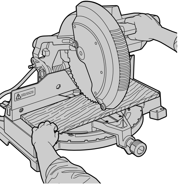
PROPER CUT
